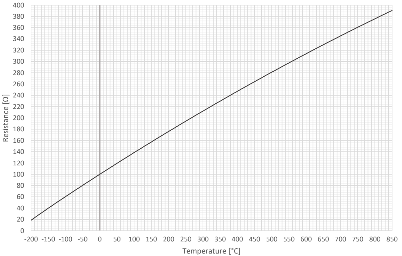
Characteristic Curve Pt100
